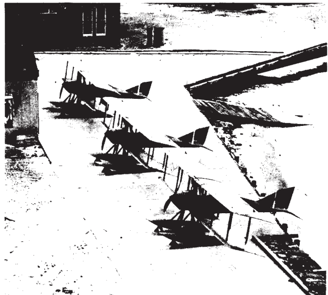
THE STURTEVANT FEATURED STEEL FRAMEWORK
