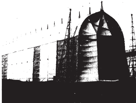
THE CANVAS BLIMP HANGAR AT NAS PAIMBOEUF
