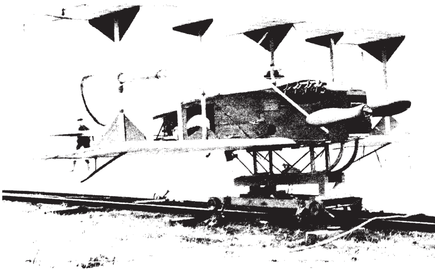
A CURTISS-SPERRY FLYING BOMB IS SHOWN HERE MOUNTED FOR A CATAPULT LAUNCH
